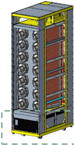
Sidecar Air Assisted Liquid Cooling(AALC) (4U RPU)
